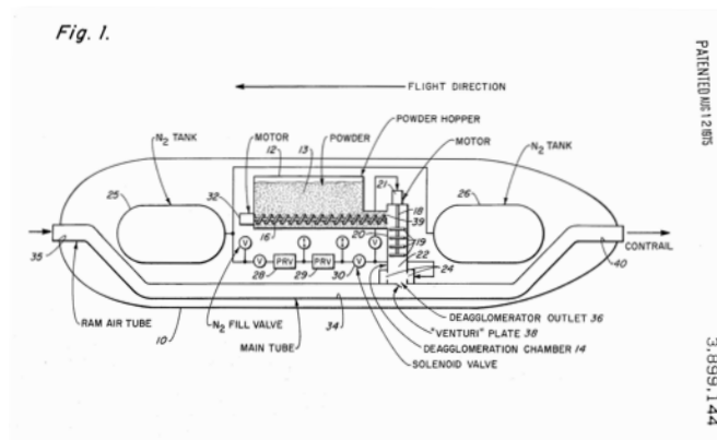
US PATENT US3899144A Powder contrail generation https://patents.google.com/patent/US3899144A/en
